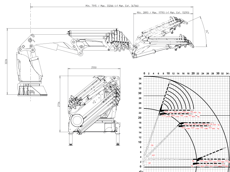
HIAB X-HIPRO 1058 E-8 + JIB 150X-6
