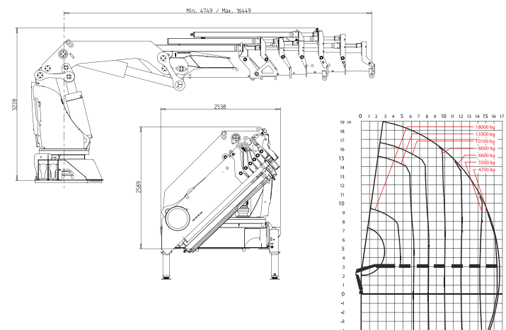
HIAB X-HIPRO 1058 E-8 + JIB 150X-6
